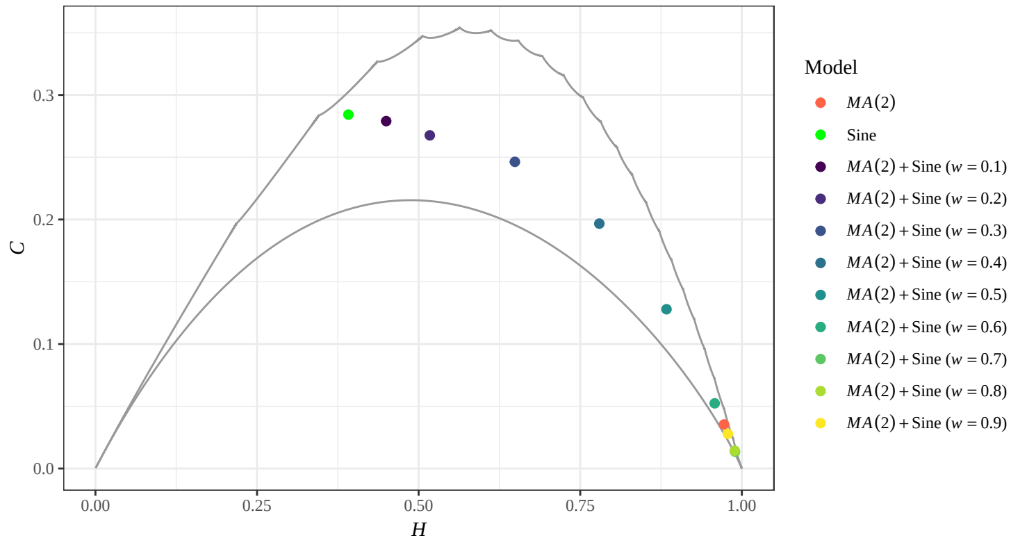
HC Plane — MA(2) + \text{Sine } (D = 4)
