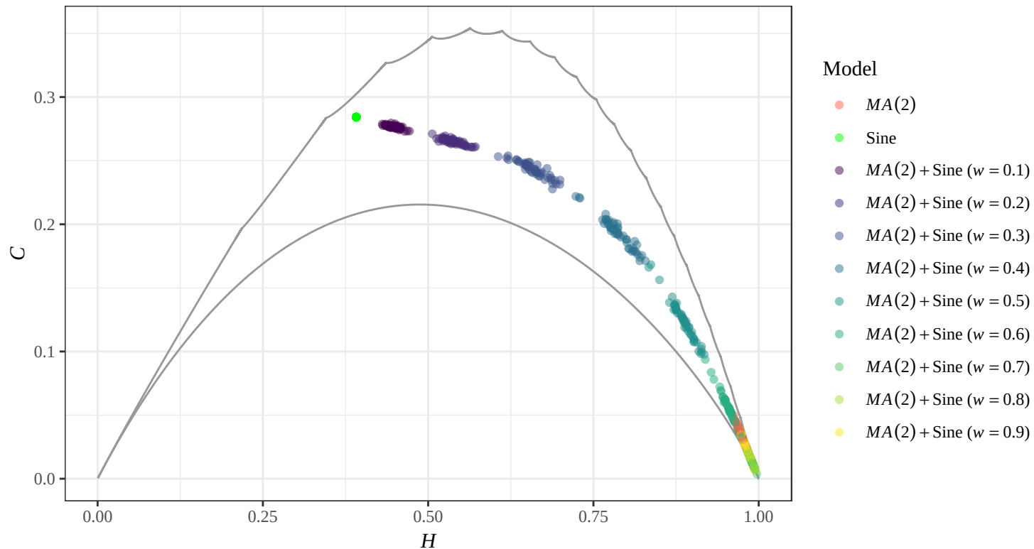
HC Plane — MA(2) + \text{Sine} (50 reps, D = 4 )
