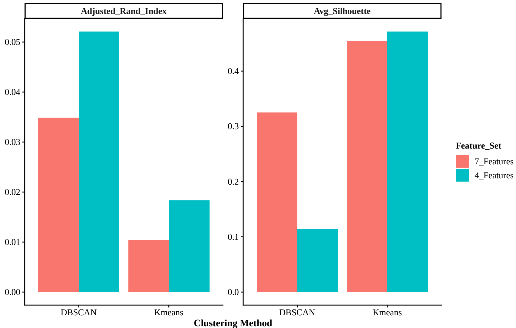
WIZ: Clustering Quality by Feature Set
