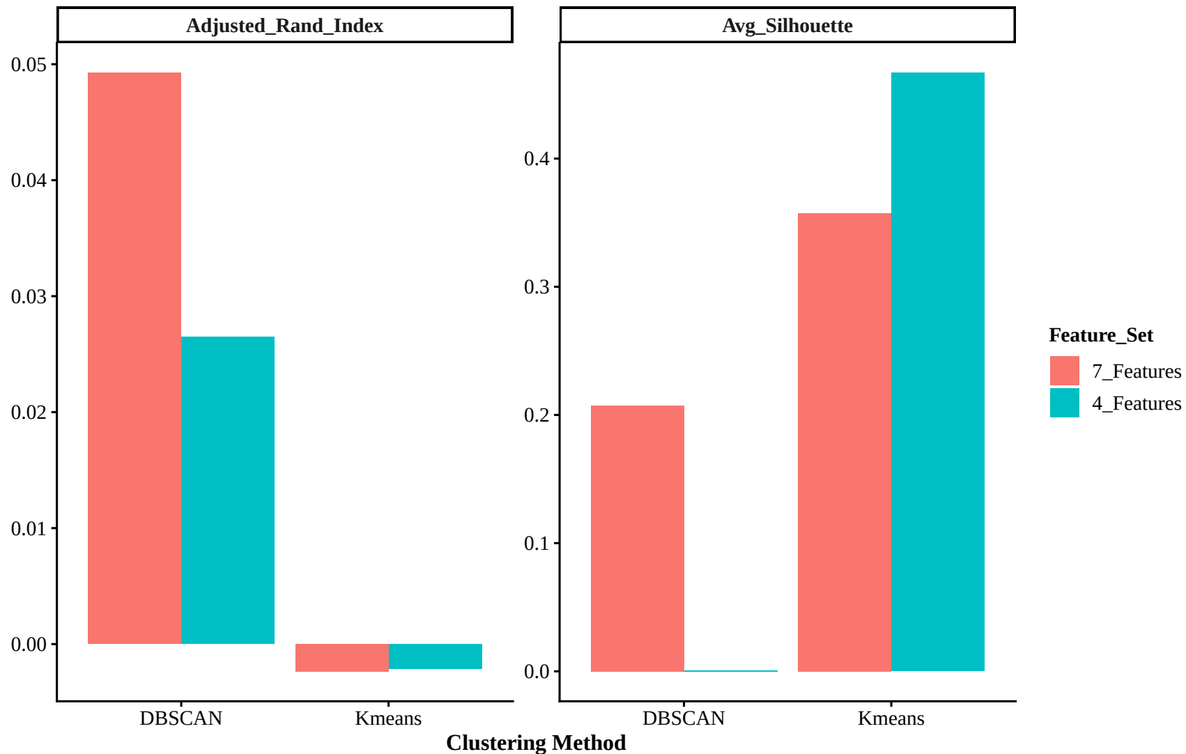
WSRZ: Clustering Quality by Feature Set
