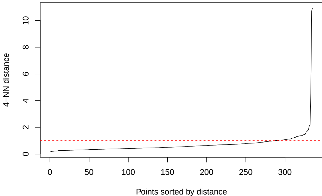
WIZ: k-NN distance plot
