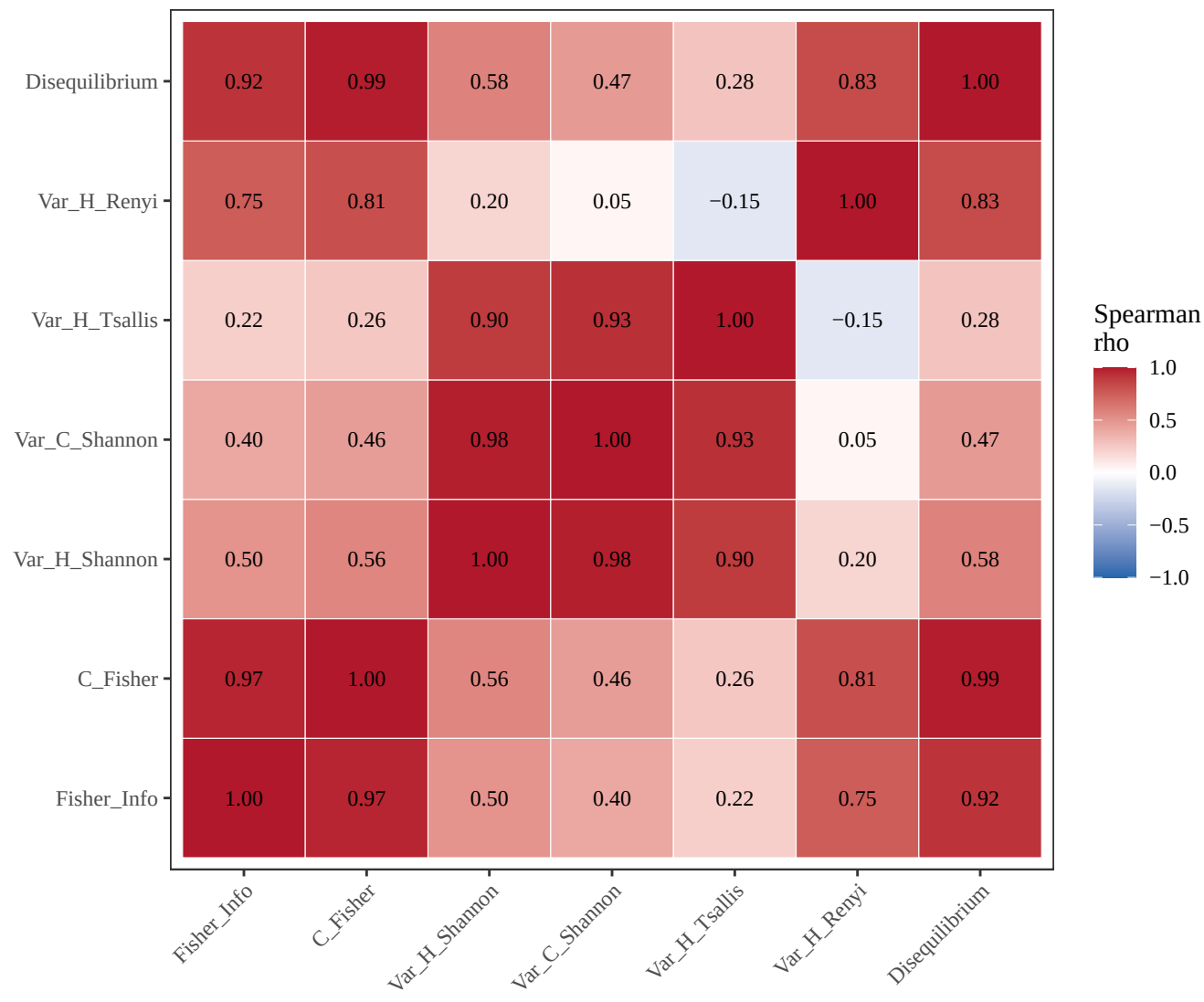
WIZ: Feature Correlation
