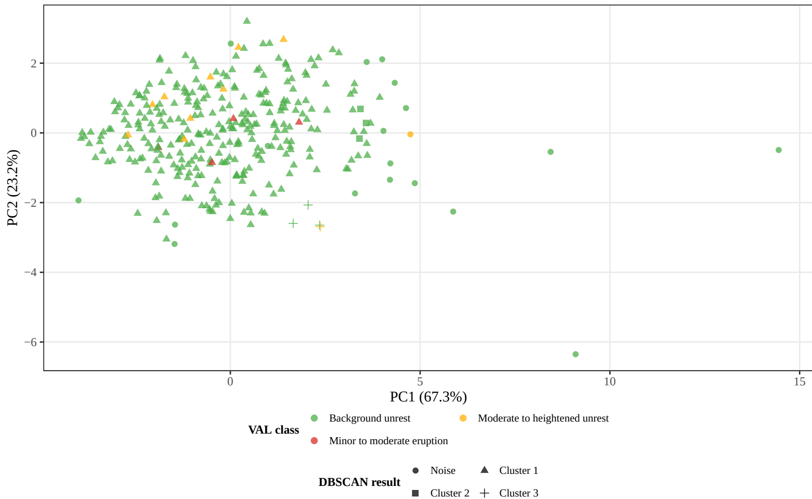
WSRZ: DBSCAN Three-Cluster Solution
