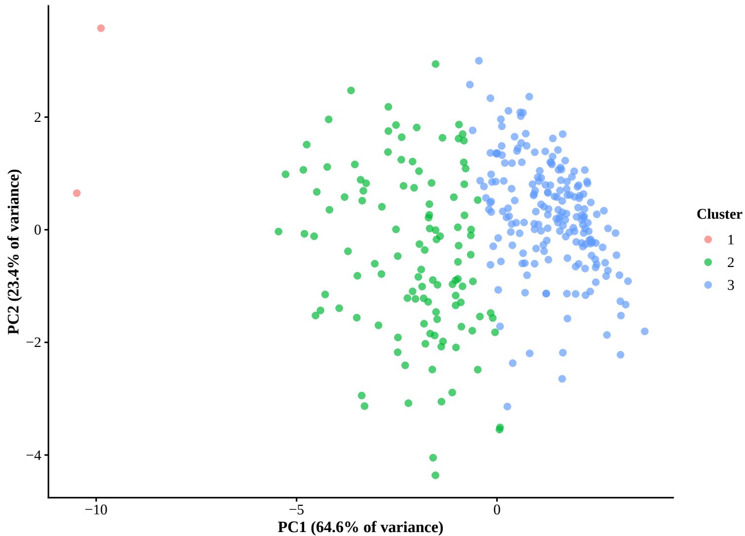
WIZ: K-means Clustering
