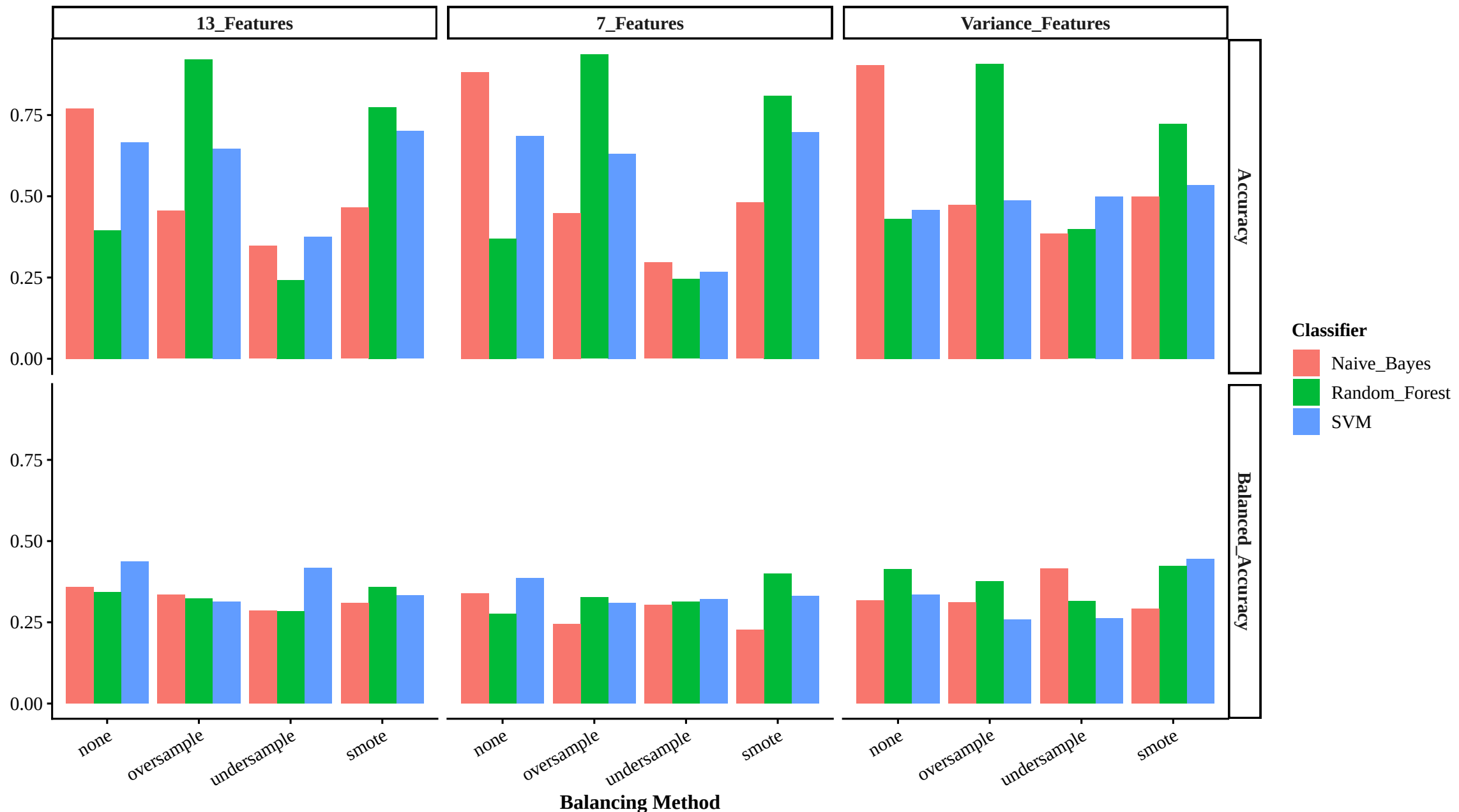
WIZ: Accuracy vs Balanced Accuracy by Feature Set and Balancing Method
