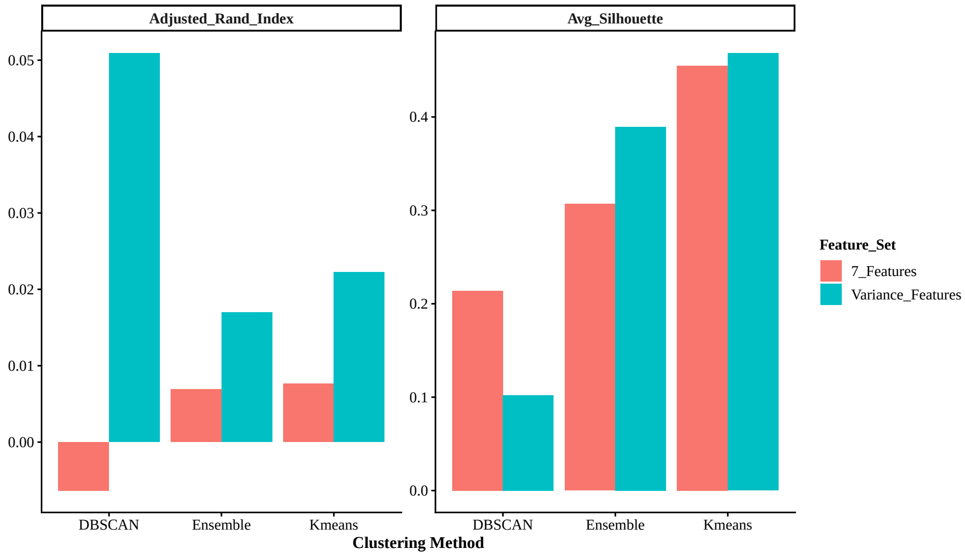
WIZ: Clustering Quality by Feature Set
