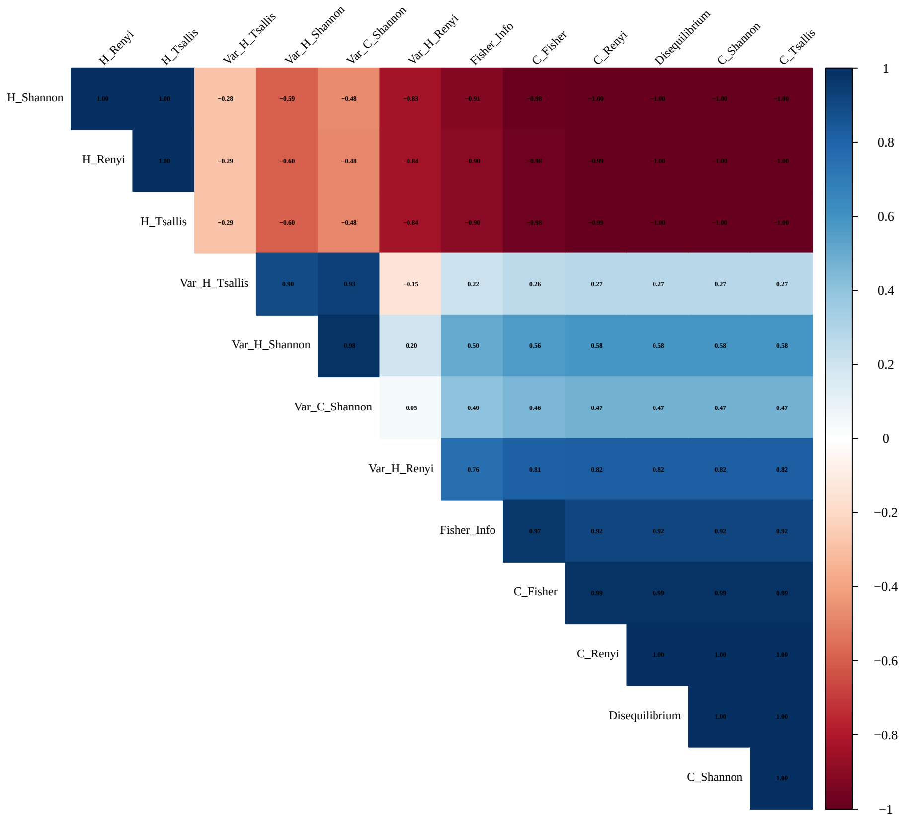
WIZ – Correlation of 13 Original Features
