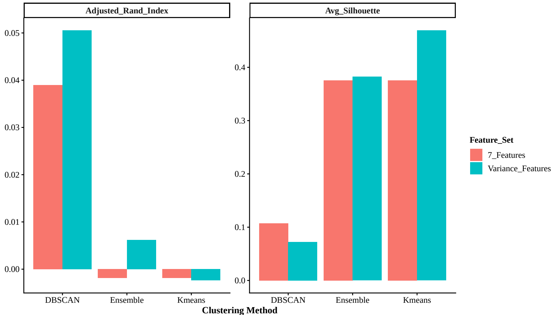
WSRZ: Clustering Quality by Feature Set
