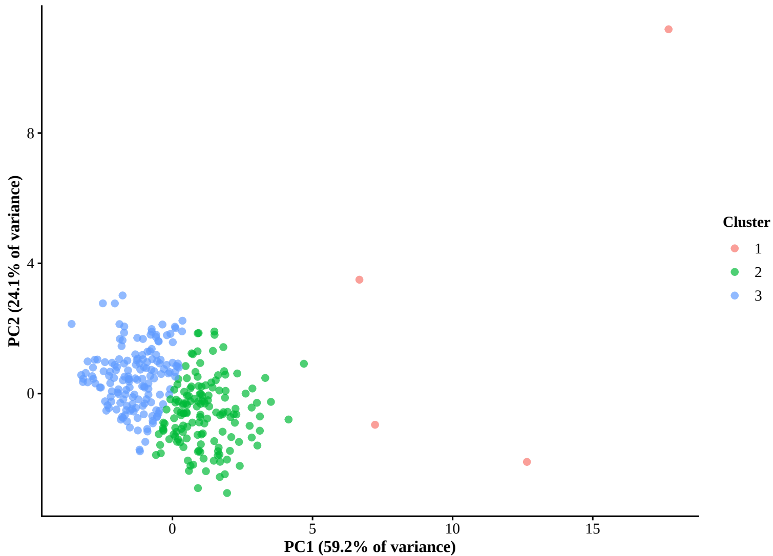
WSRZ: K-means Clustering
