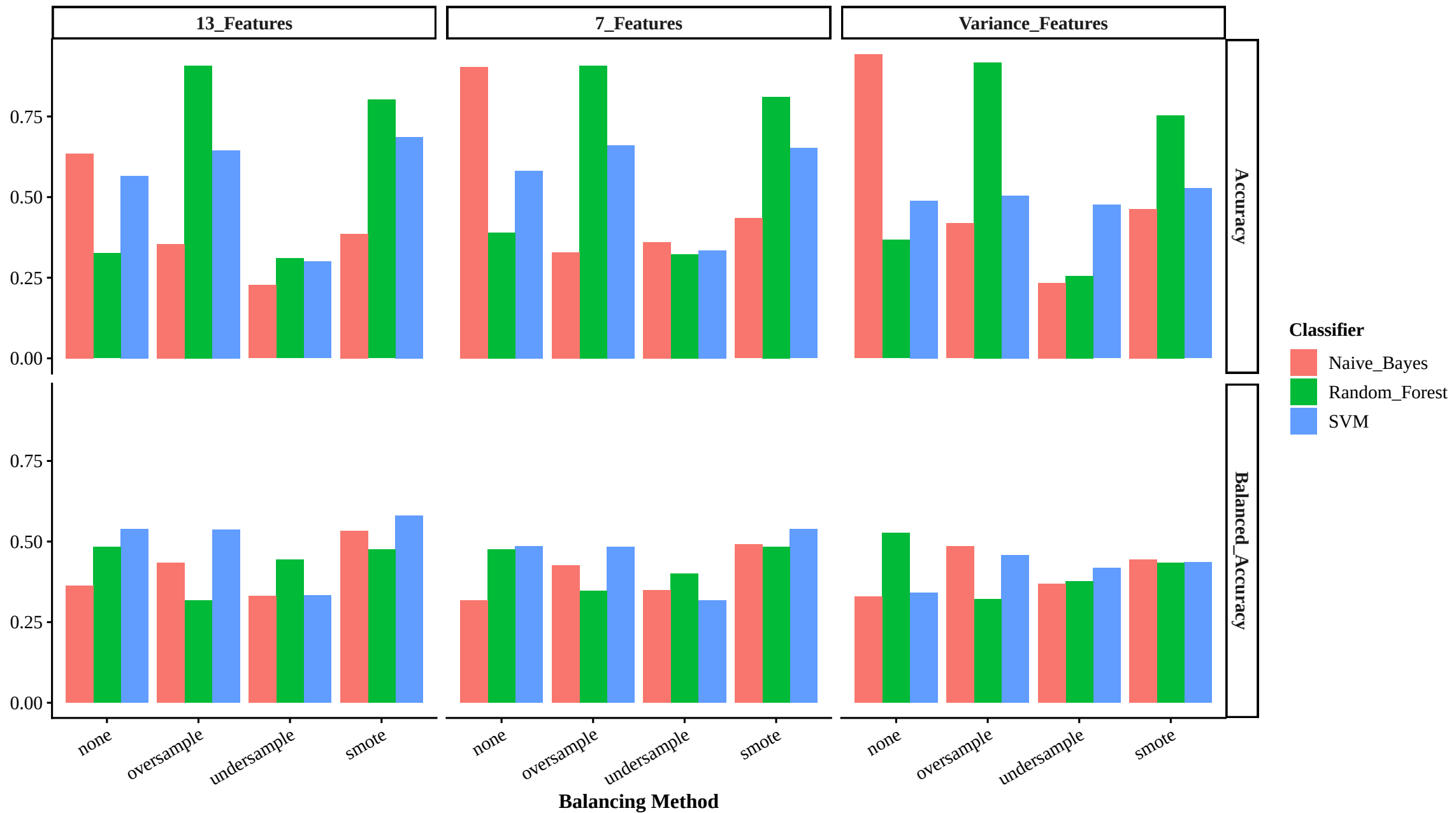
WSRZ: Accuracy vs Balanced Accuracy by Feature Set and Balancing Method
