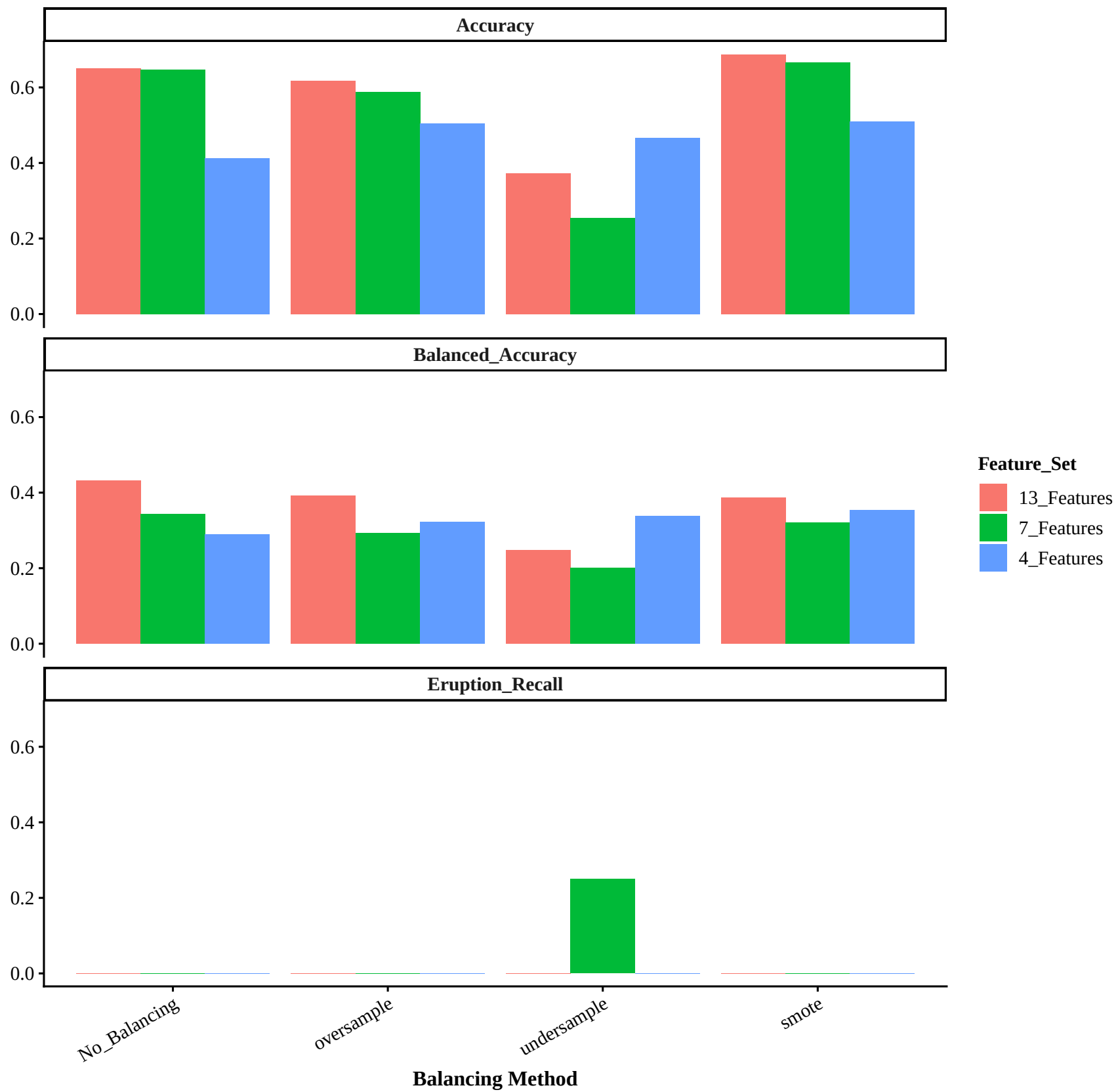
WIZ: SVM Performance by Feature Set and Balancing Method
