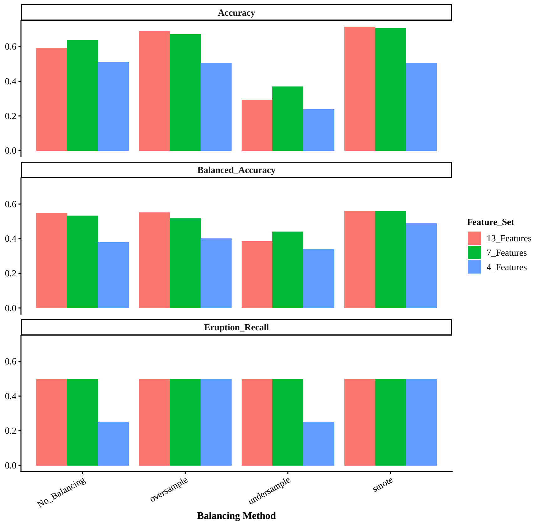
WSRZ: SVM Performance by Feature Set and Balancing Method
