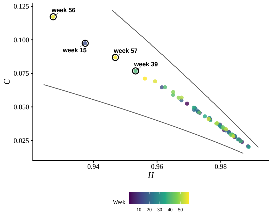
RSAM Shannon H \times C plane
