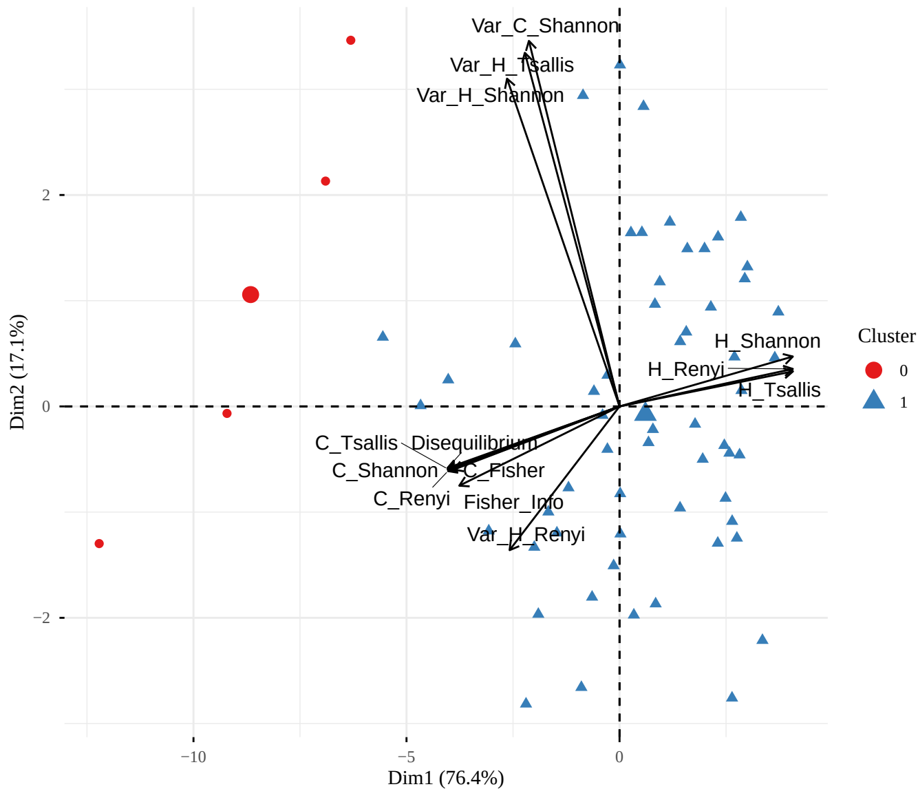
PCA biplot: weeks (by DBSCAN cluster) and feature loadings
