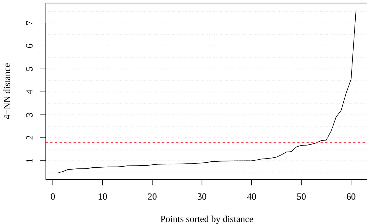
k-NN distance plot (k = 4) -- eps = 1.80
