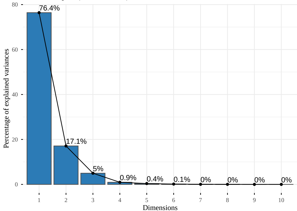
PCA scree plot (RSAM, 2019)
