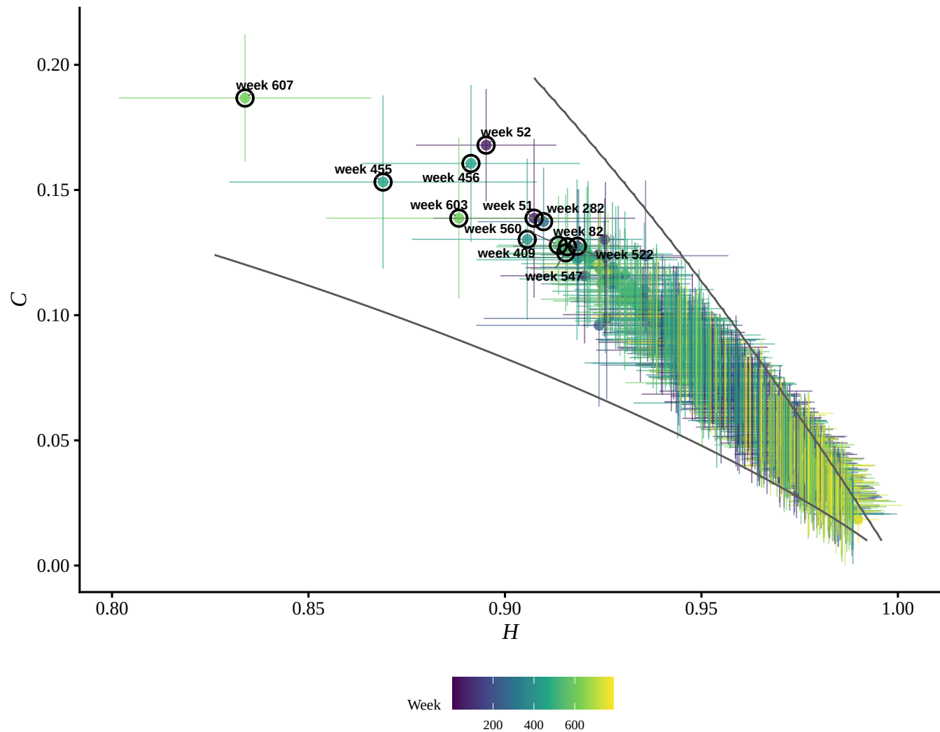
RSAM 2007 to 2019 Shannon H \times C plane
