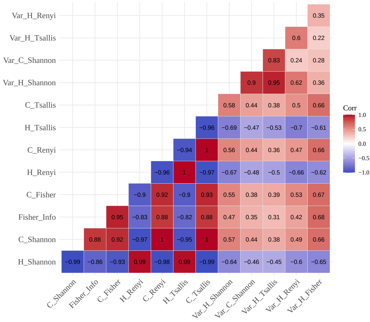
Correlation of H-C Features (RSAM, 2007–2019)
