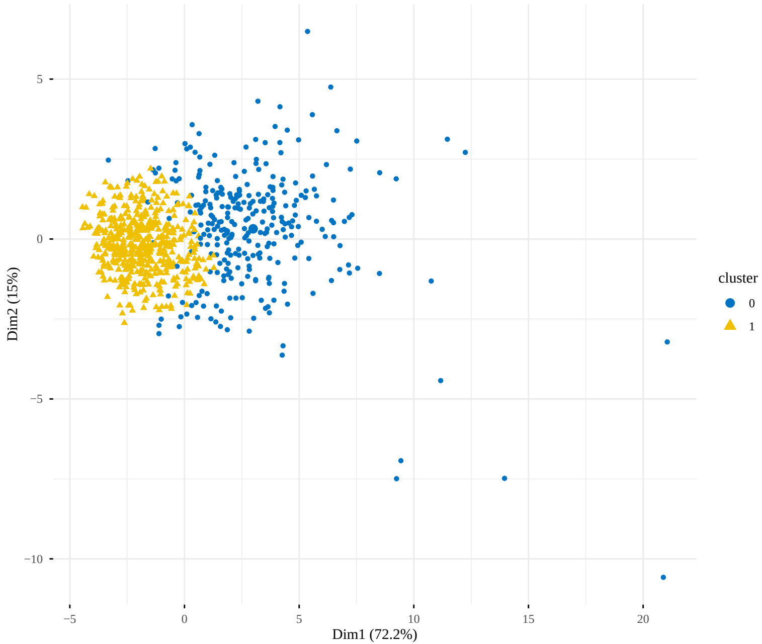
DBSCAN Clustering (eps = 1, minPts = 26)
