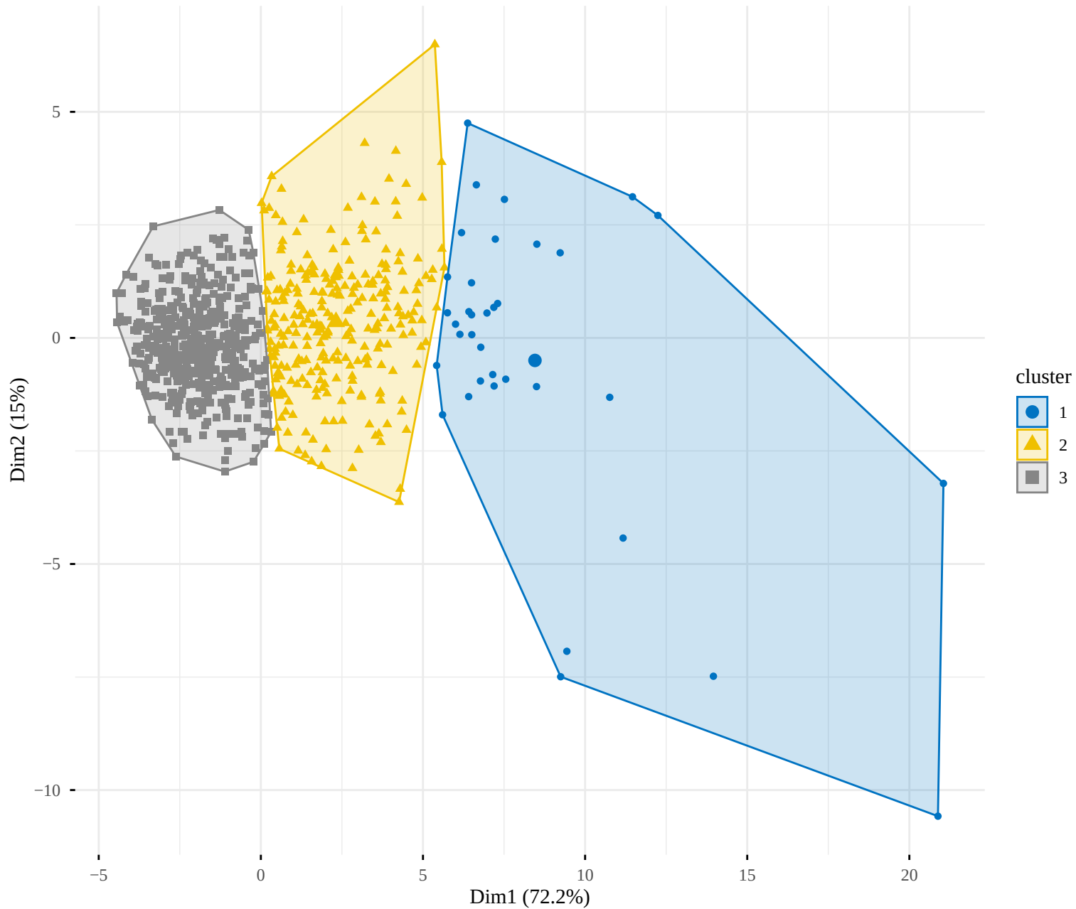
K-means Clustering (k = 3)
