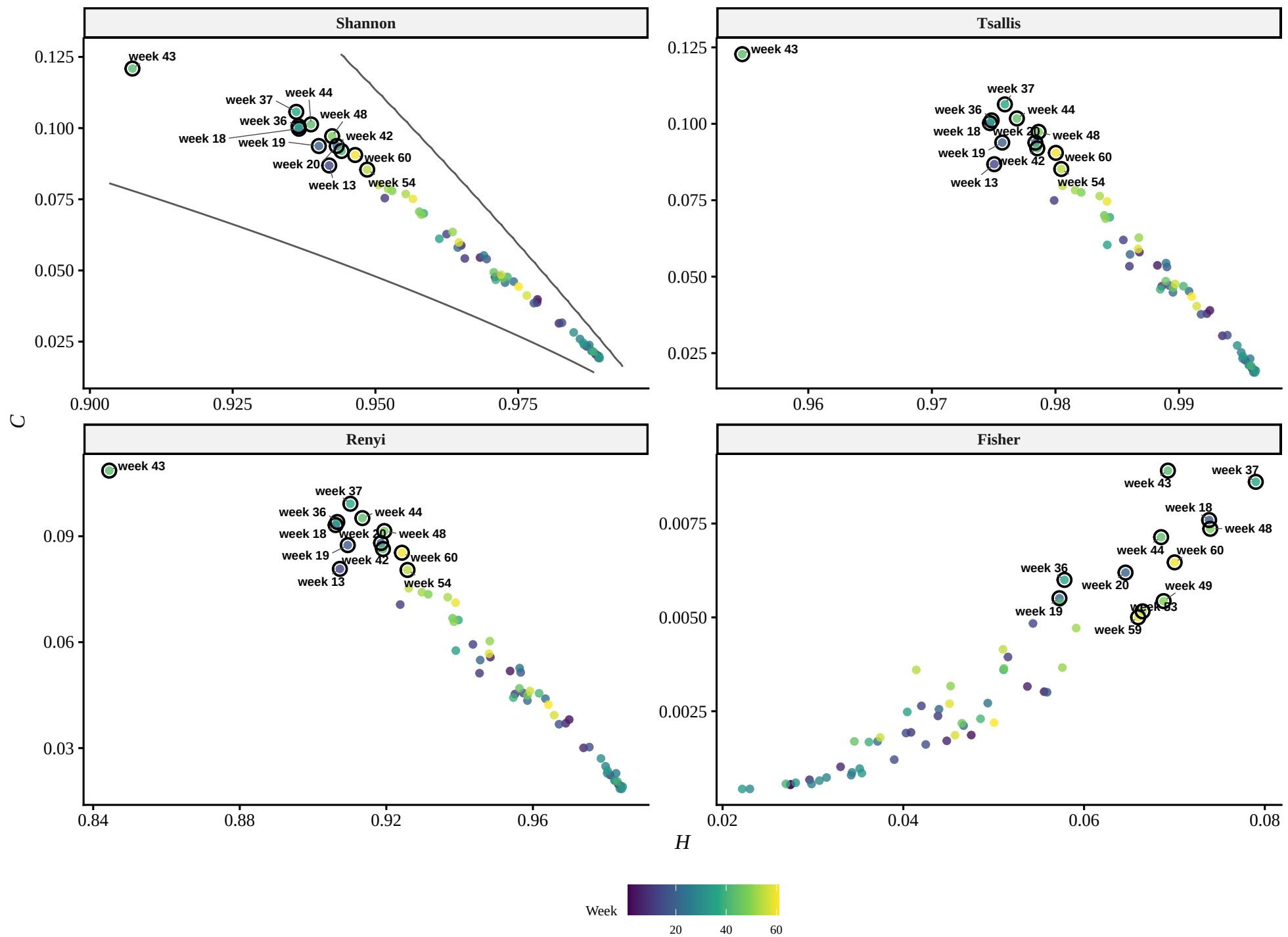
RSAM 2013 H \times C plane
