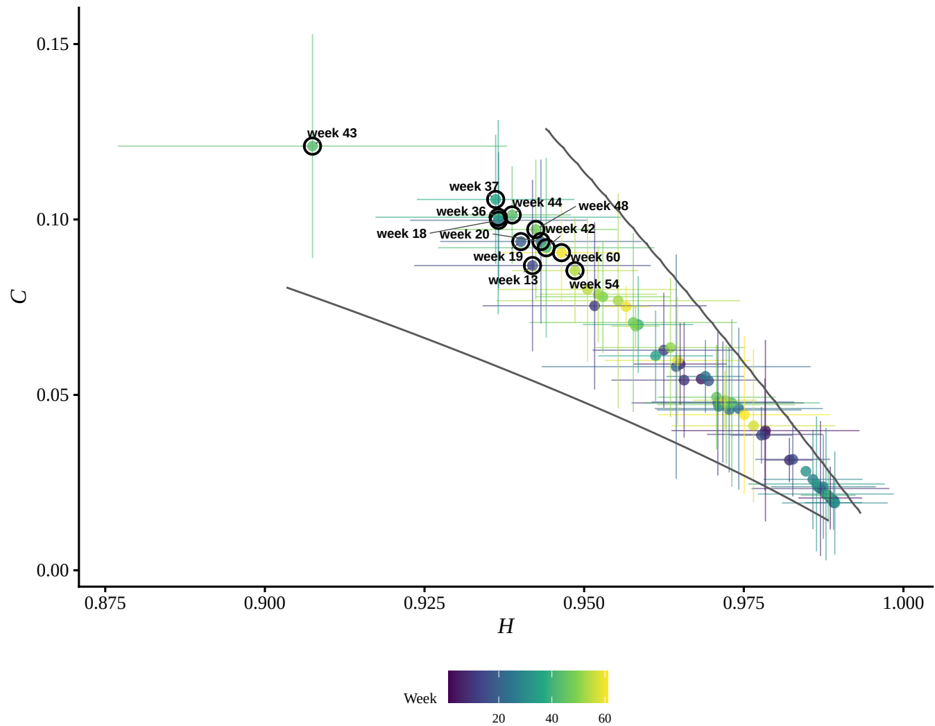
RSAM 2013 Shannon H \times C plane
