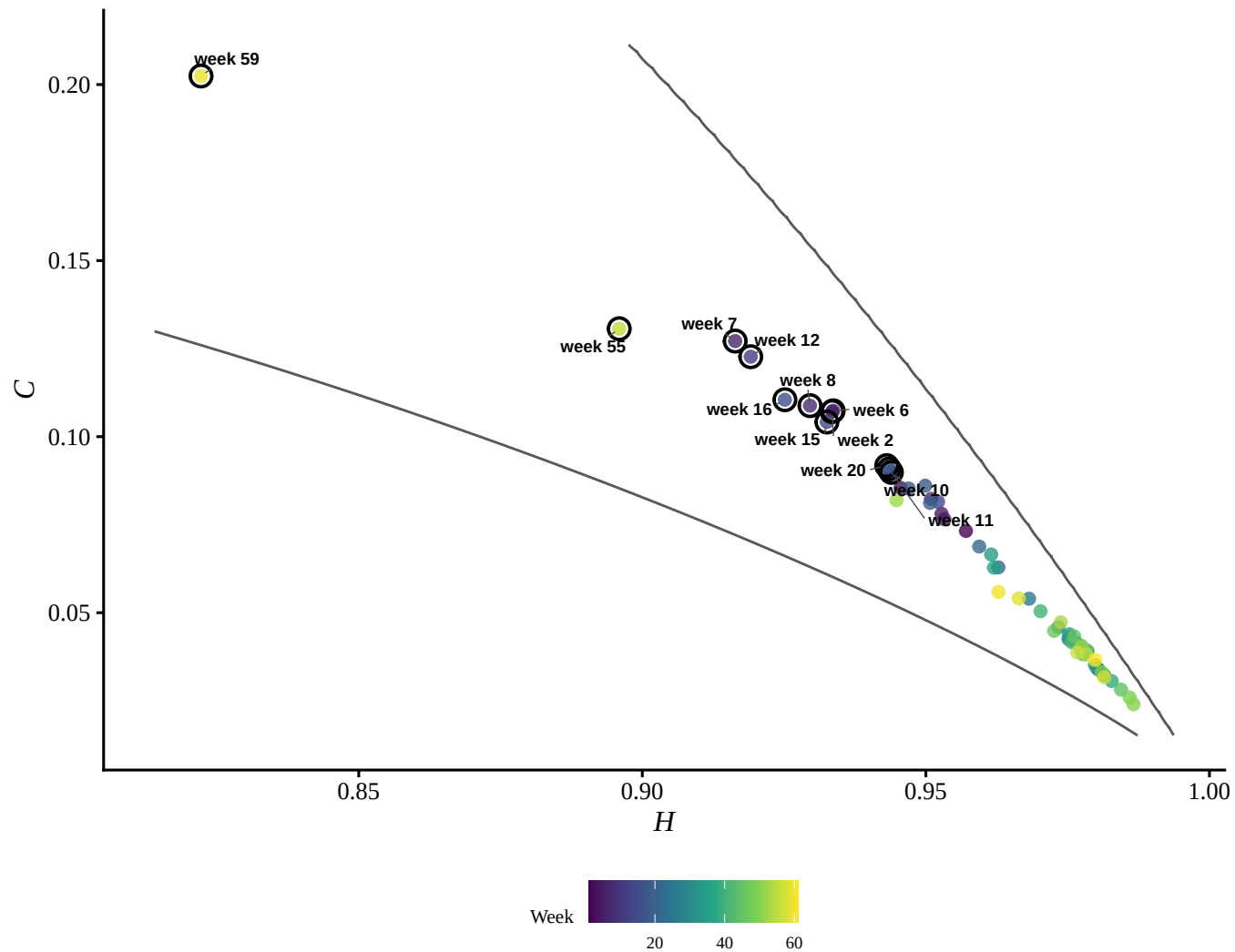
RSAM 2016 Shannon H \times C plane
