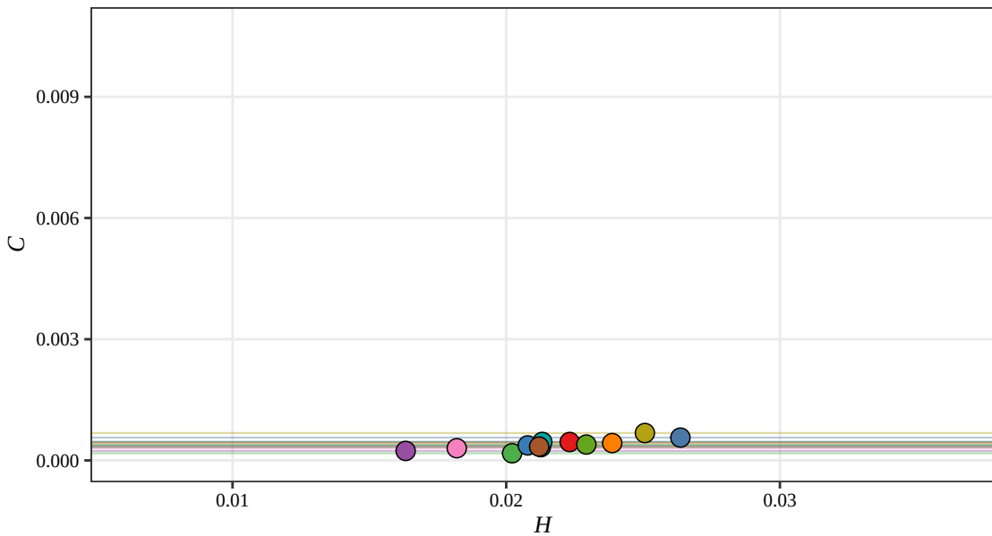
Fisher H-C Plane, D = 5 (Displacement, 2011)
