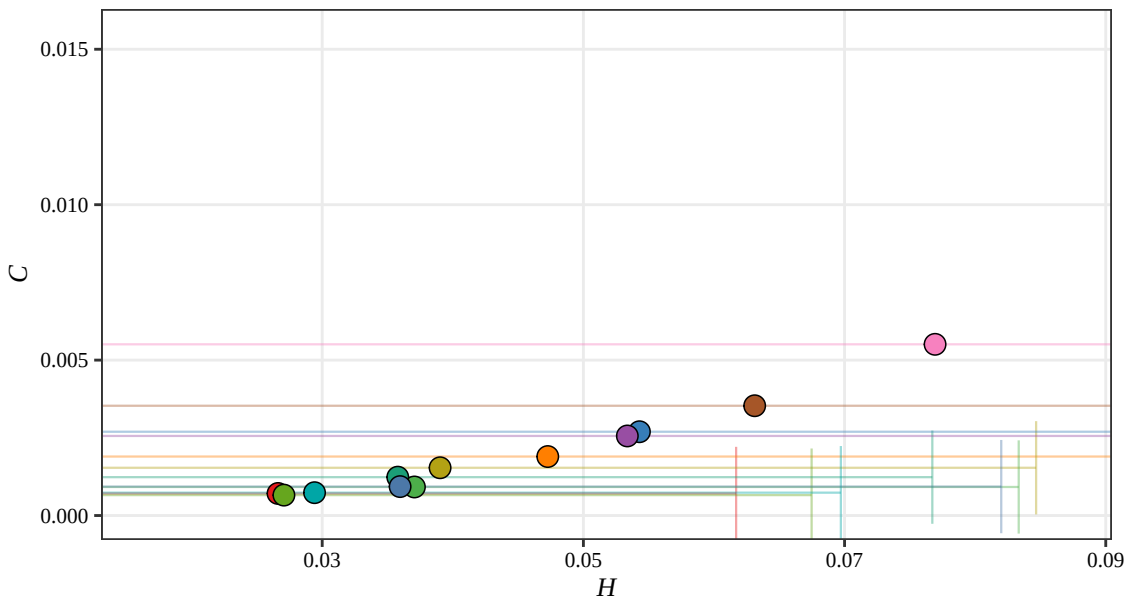
Fisher H-C Plane, D = 5 (RSAM, 2011)
