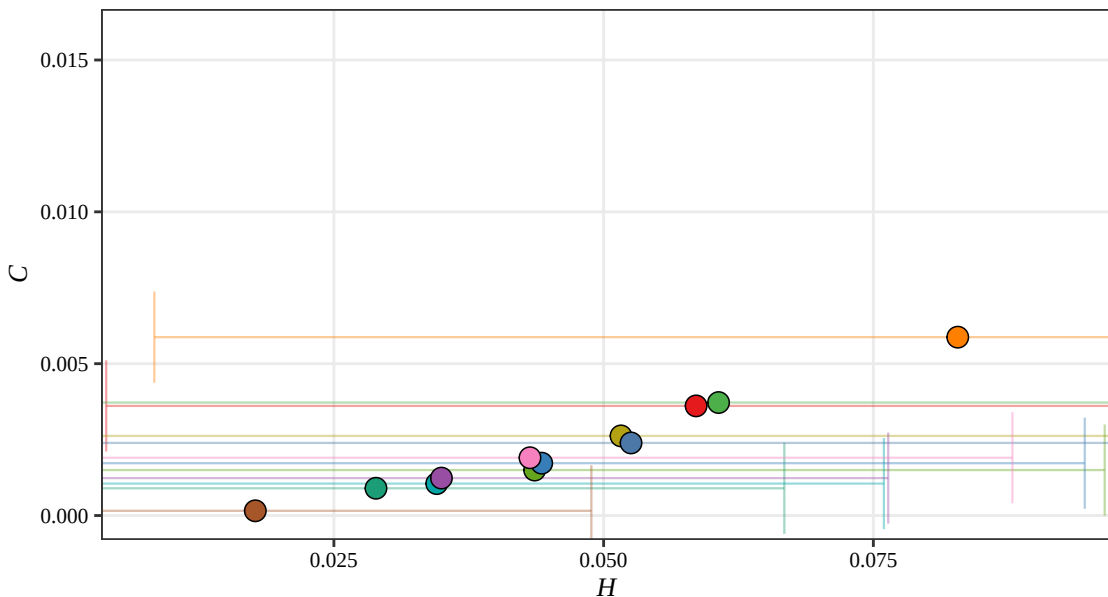
Fisher H-C Plane, D = 5 (RSAM, 2012)
