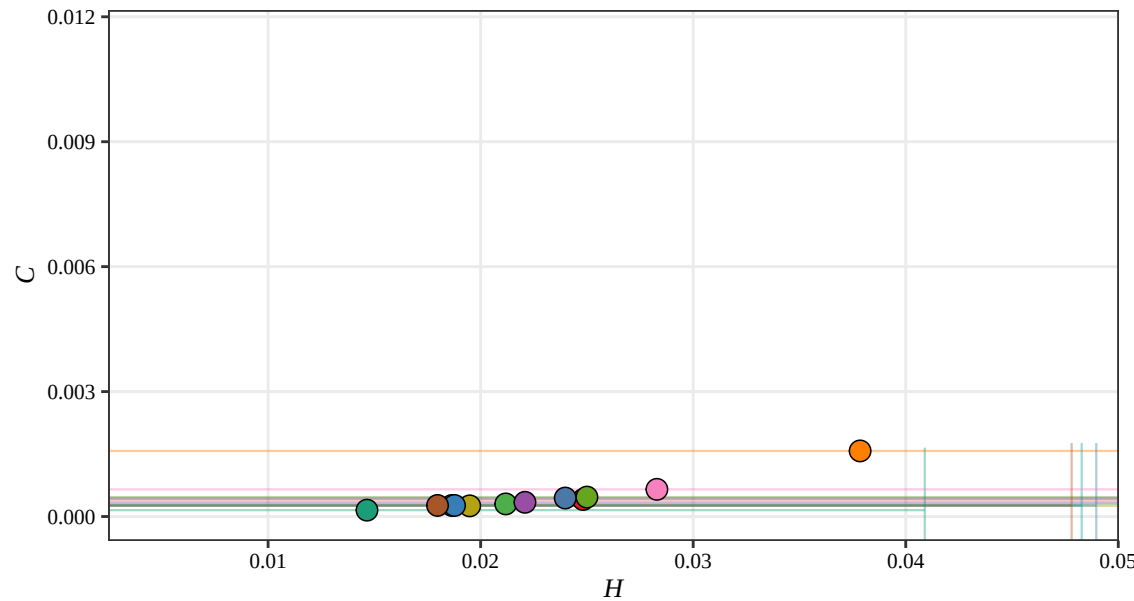
Fisher H-C Plane, D = 5 (Displacement, 2013)
