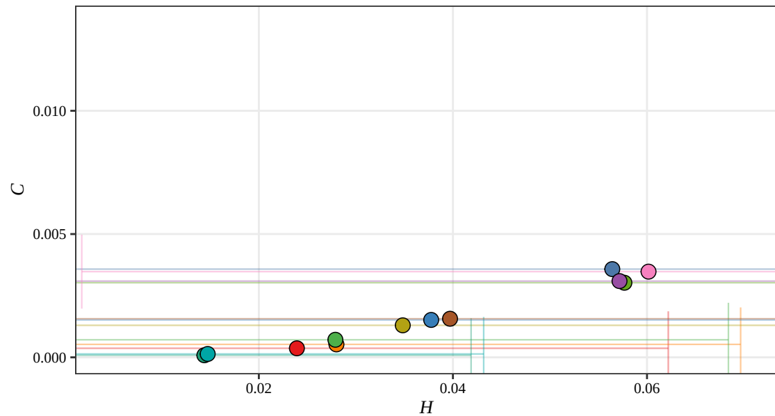
Fisher H-C Plane, D = 5 (RSAM, 2013)
