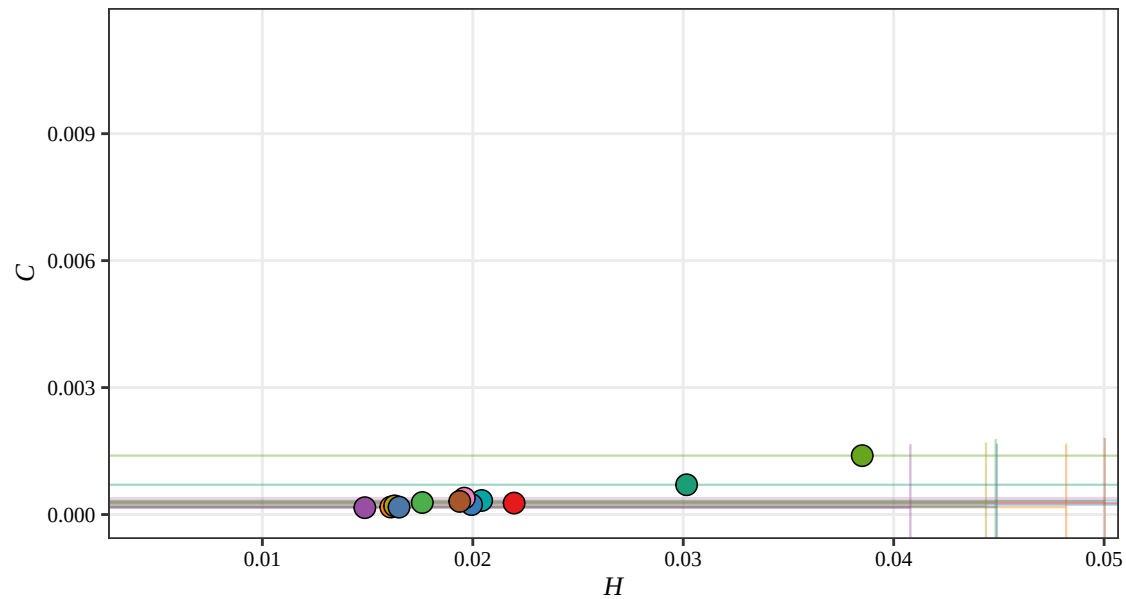
Fisher H-C Plane, D = 5 (Displacement, 2014)
