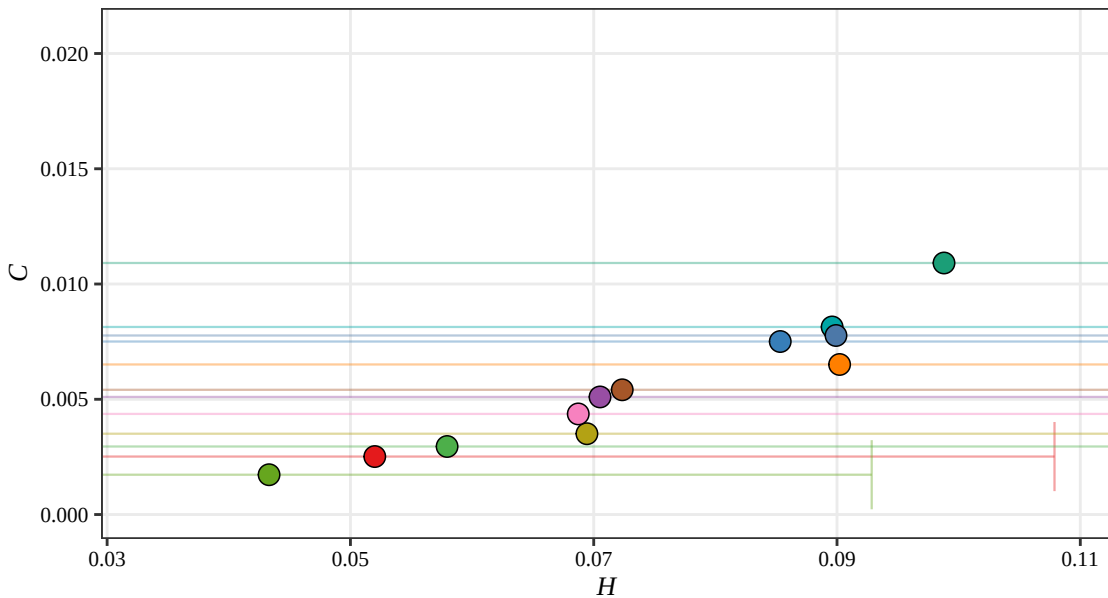
Fisher H-C Plane, D = 5 (RSAM, 2014)
