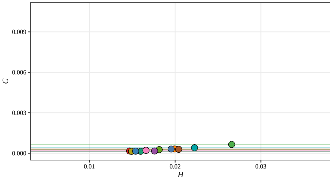
Fisher H-C Plane, D = 5 (Displacement, 2015)
