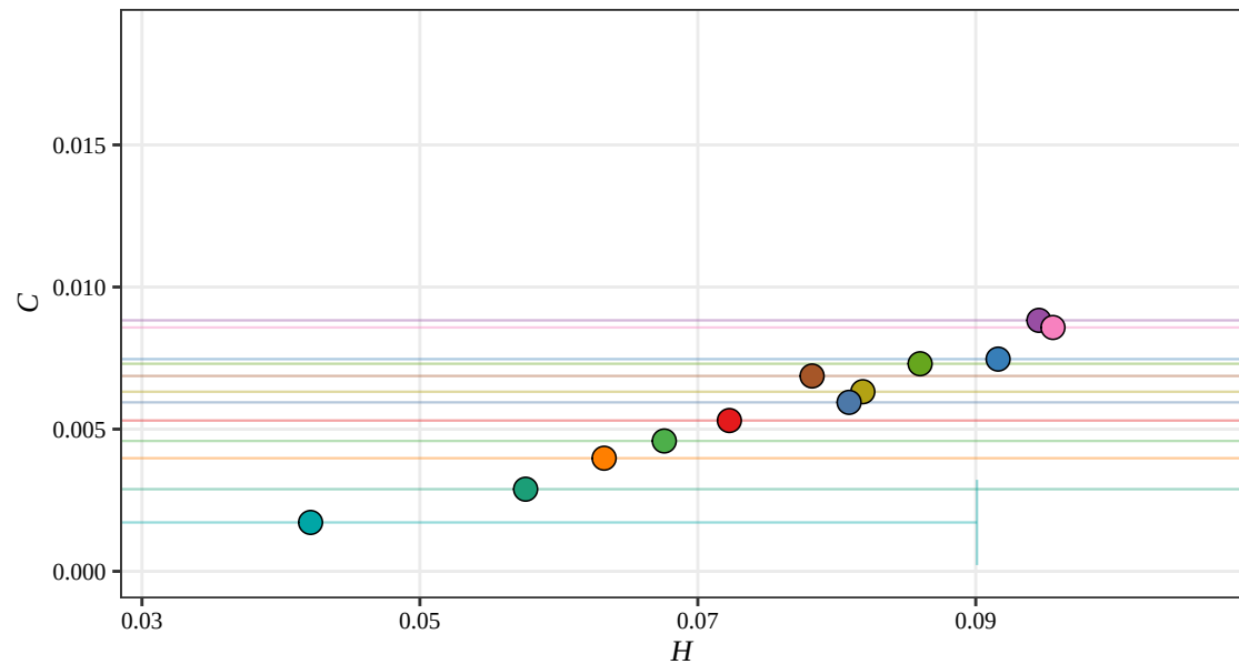
Fisher H-C Plane, D = 5 (RSAM, 2015)
