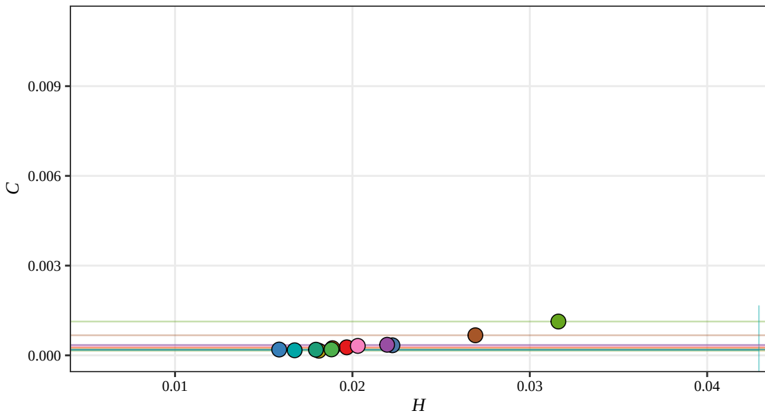
Fisher H-C Plane, D = 5 (Displacement, 2016)
