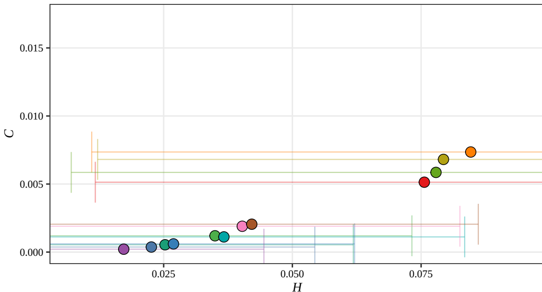
Fisher H-C Plane, D = 5 (RSAM, 2016)
