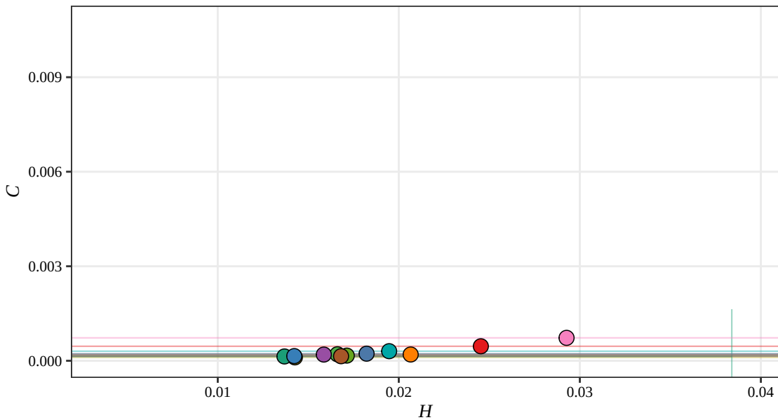
Fisher H-C Plane, D = 5 (Displacement, 2017)
