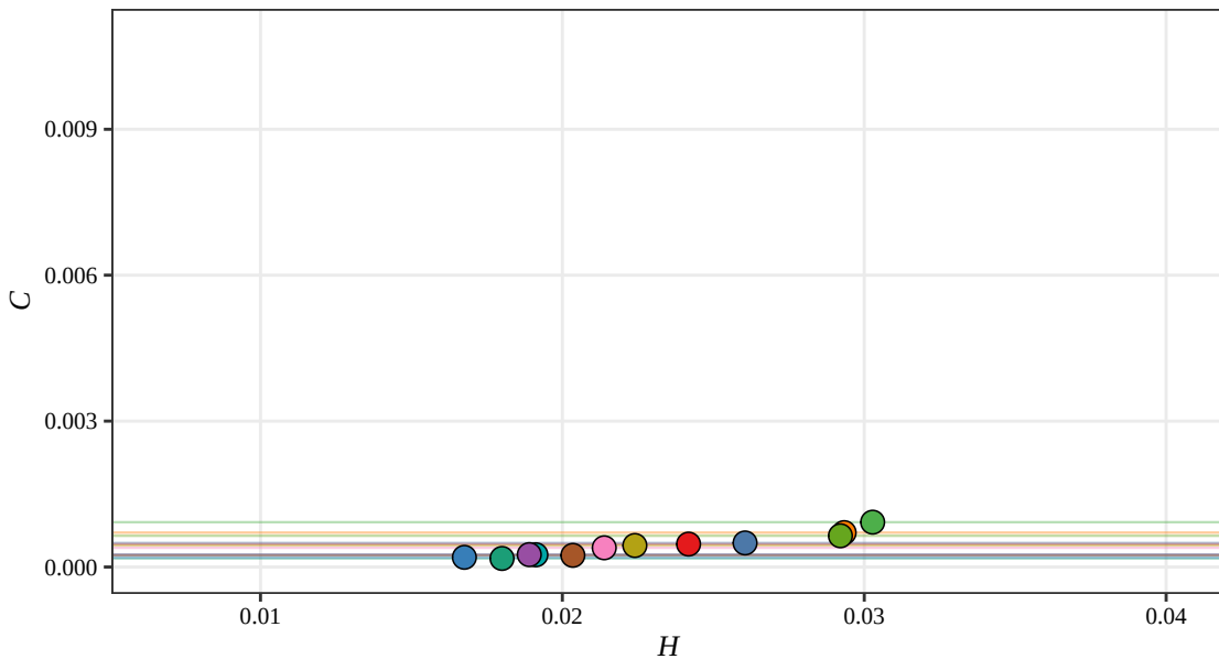
Fisher H-C Plane, D = 5 (RSAM, 2017)
