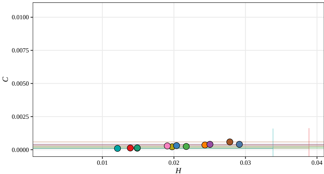
Fisher H-C Plane, D = 5 (Displacement, 2018)
