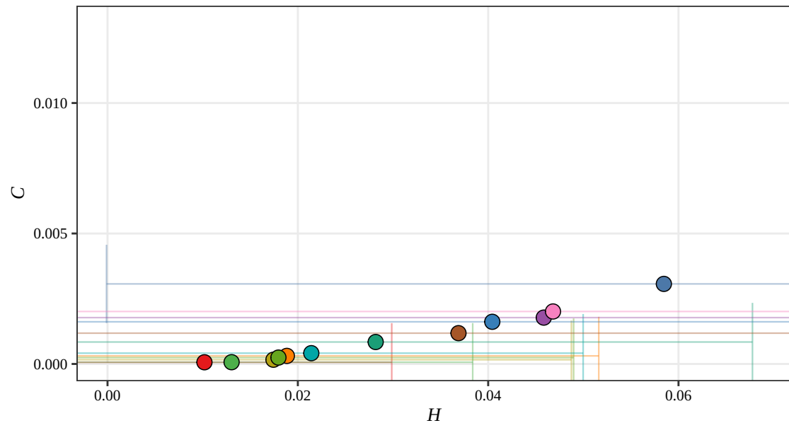
Fisher H-C Plane, D = 5 (RSAM, 2018)
