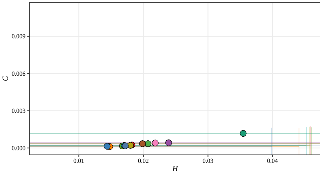
Fisher H-C Plane, D = 5 (Displacement, 2019)
