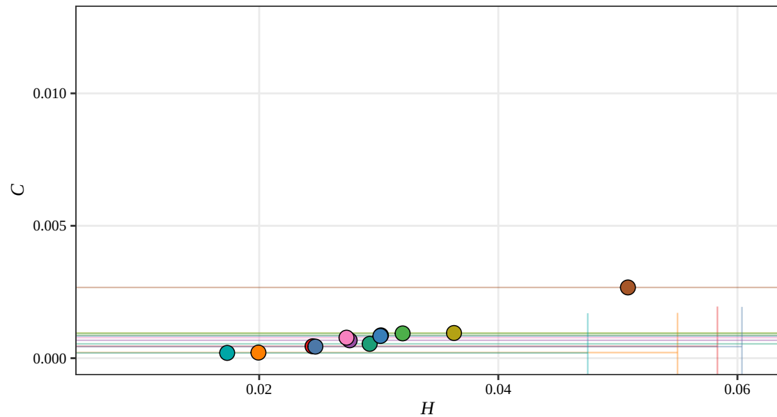
Fisher H-C Plane, D = 5 (RSAM, 2019)
