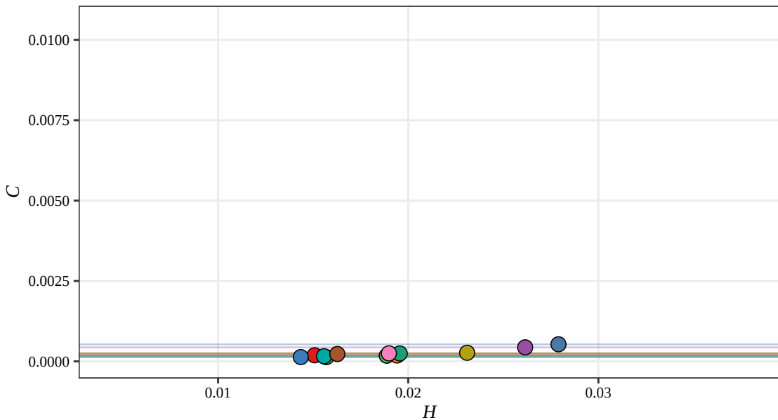
Fisher H-C Plane, D = 5 (Displacement, 2020)
