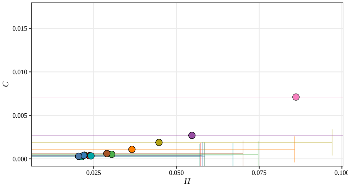
Fisher H-C Plane, D = 5 (Displacement, 2021)
