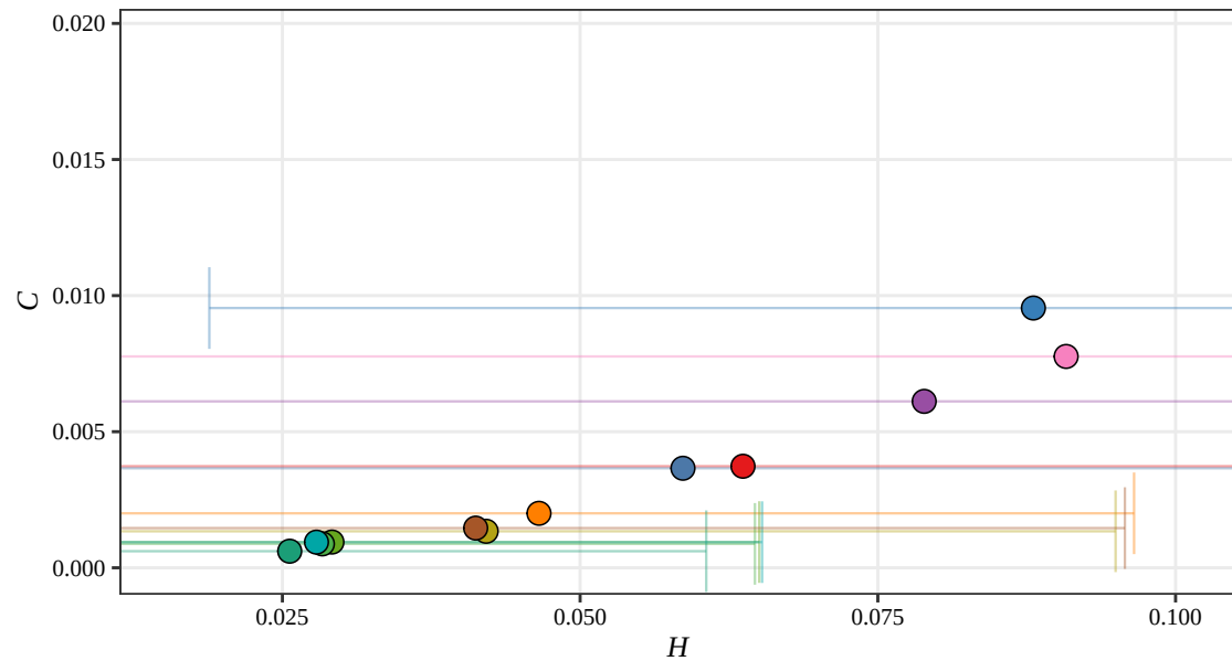
Fisher H-C Plane, D = 5 (RSAM, 2021)
