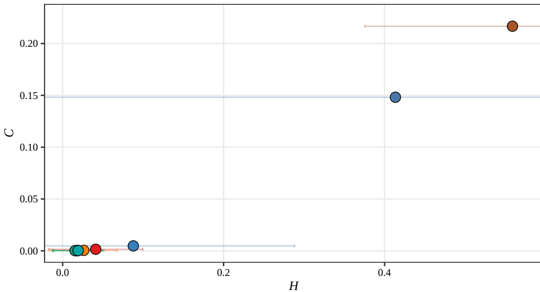
Fisher H-C Plane, D = 5 (Displacement, 2022)
