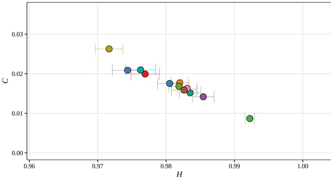
Rényi H-C Plane, D = 5 (Displacement, 2011)
