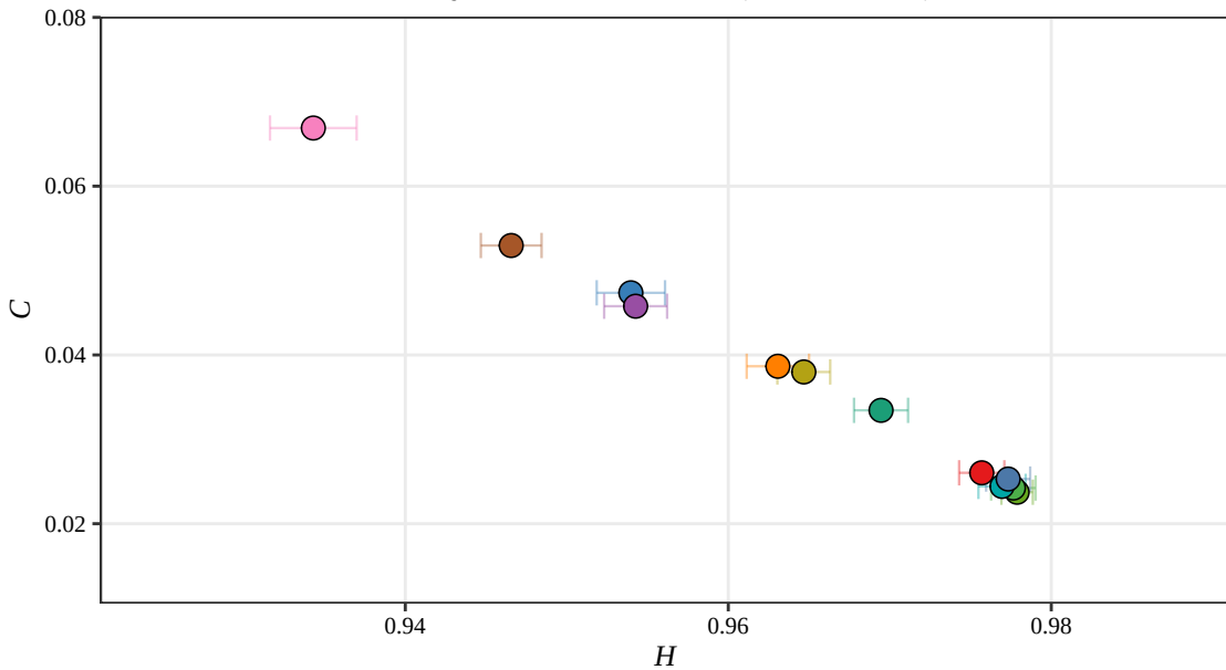
Rényi H-C Plane, D = 5 (RSAM, 2011)
