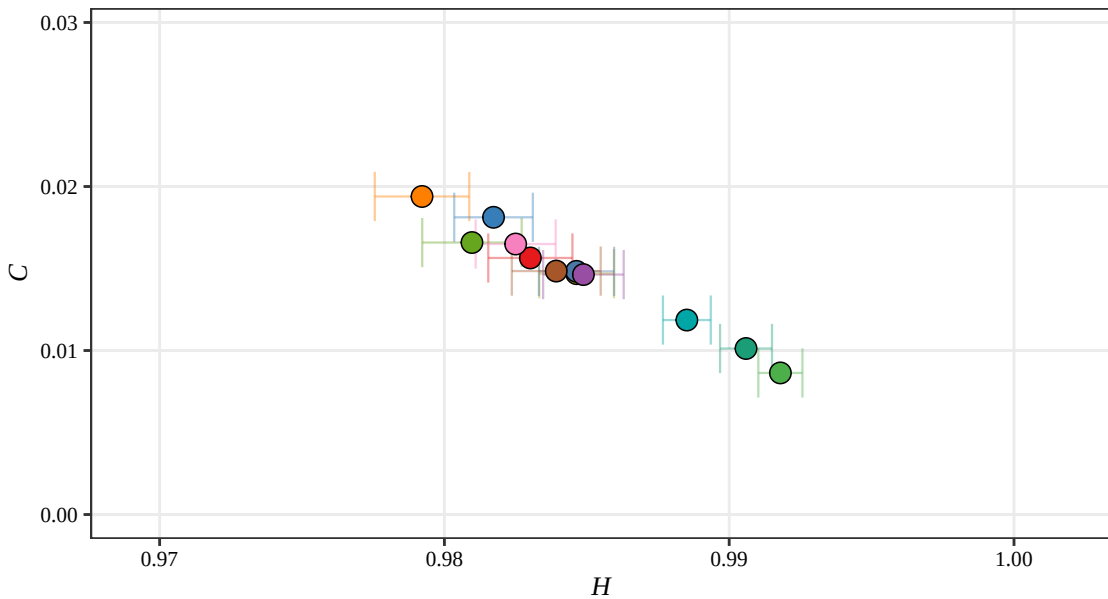
Rényi H-C Plane, D = 5 (Displacement, 2012)
