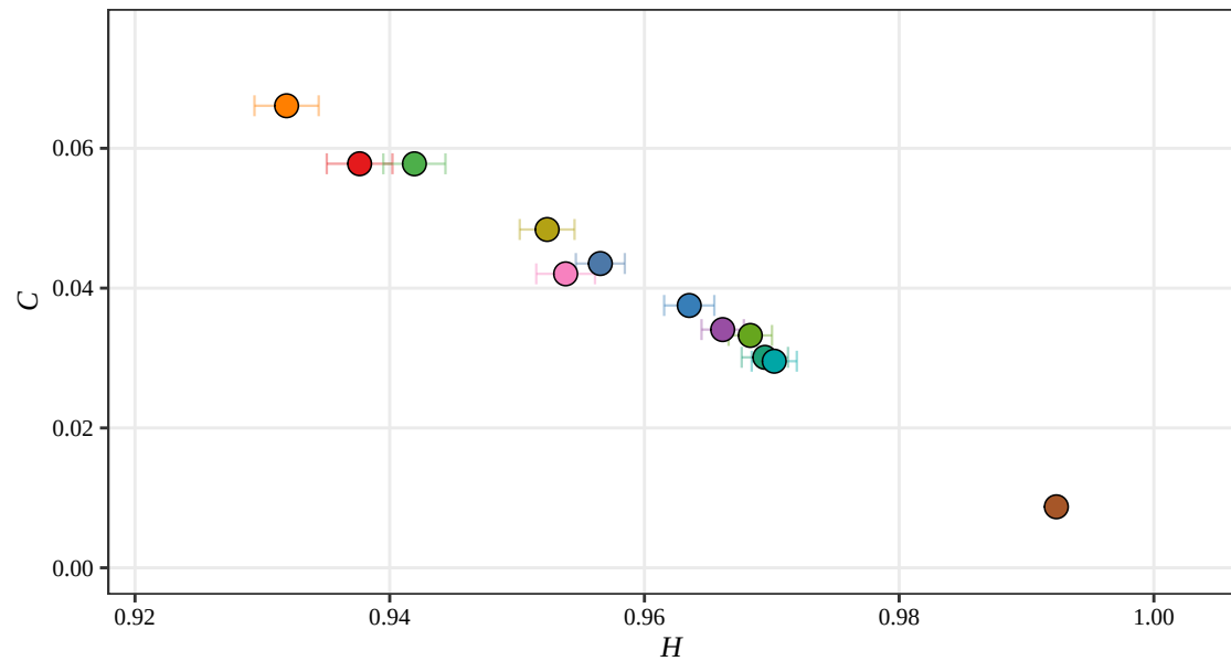
Rényi H-C Plane, D = 5 (RSAM, 2012)
