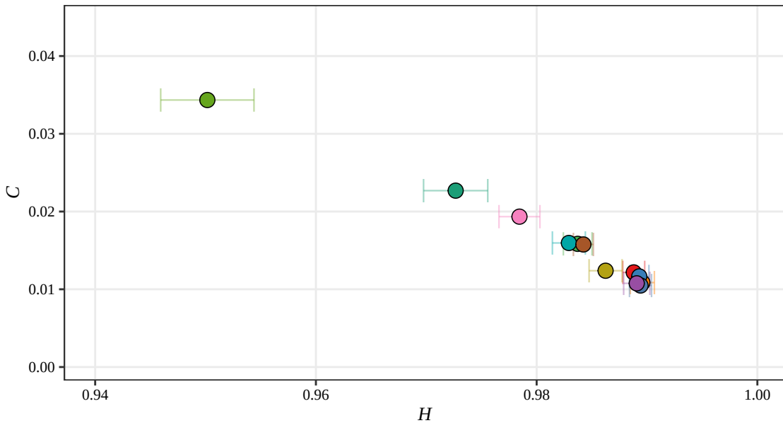
Rényi H-C Plane, D = 5 (Displacement, 2014)
