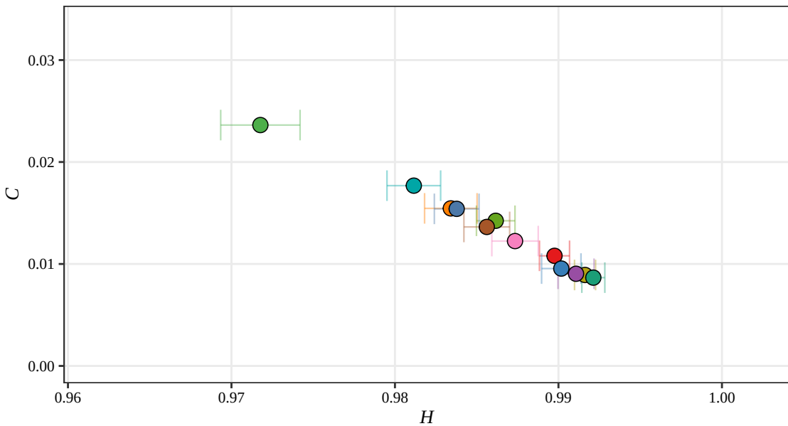
Rényi H-C Plane, D = 5 (Displacement, 2015)
