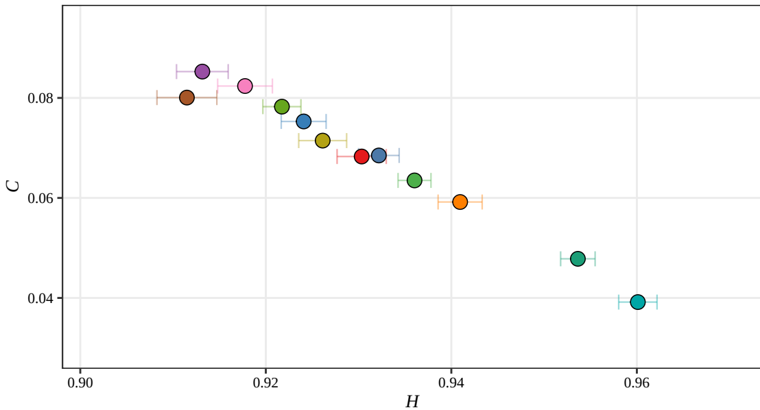
Rényi H-C Plane, D = 5 (RSAM, 2015)
